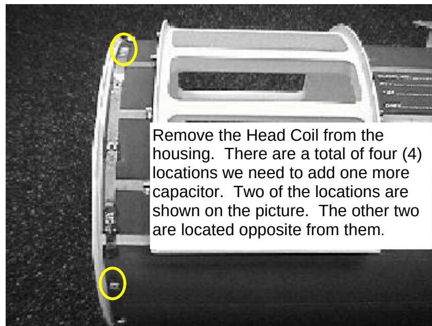
CAPACITOR LOCATIONS - SIDE VIEW ILLUSTRATION 5-3
