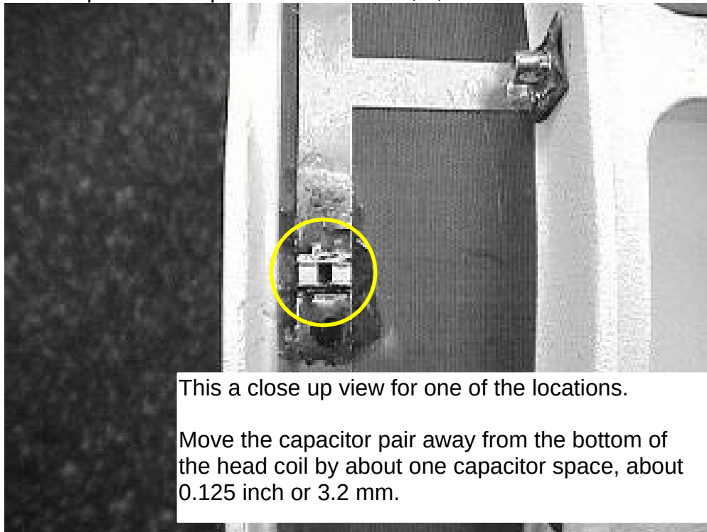
CAPACITOR LOCATION - START
