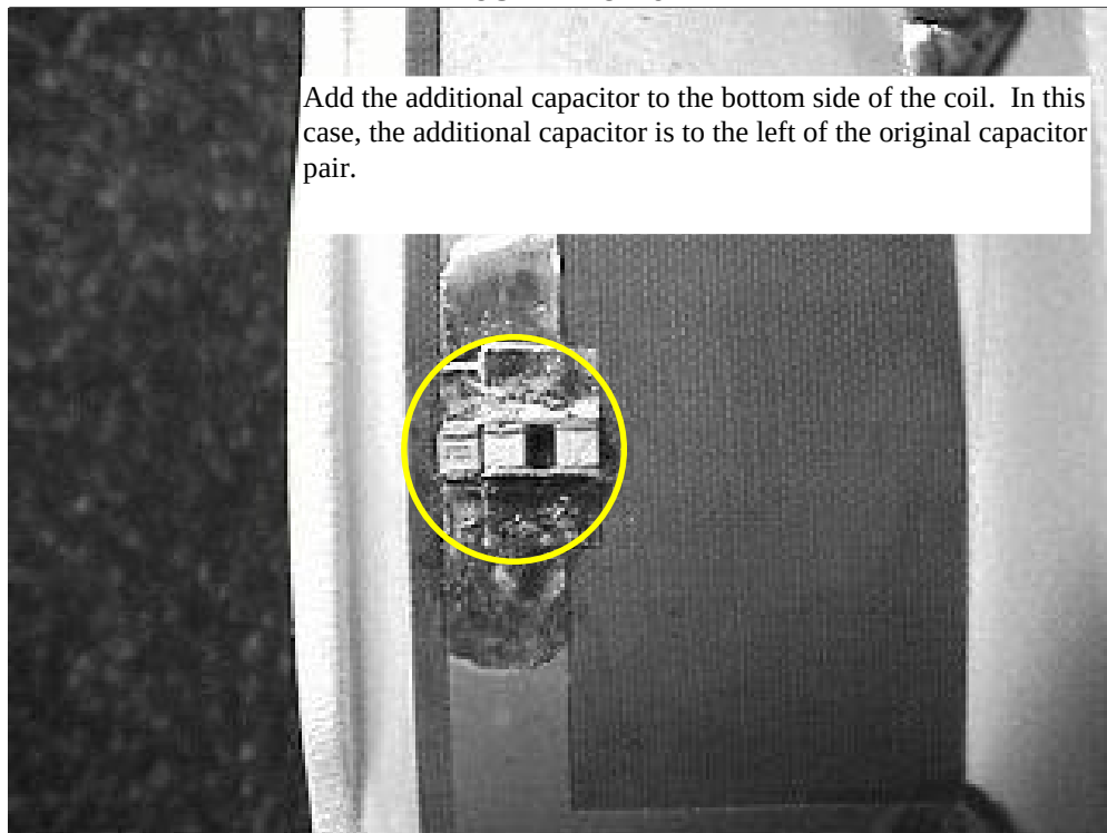
CAPACITOR LOCATION - FINISH
