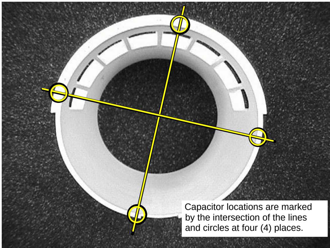
CAPACITOR LOCATIONS - BOTTOM VIEW ILLUSTRATION 5-2
