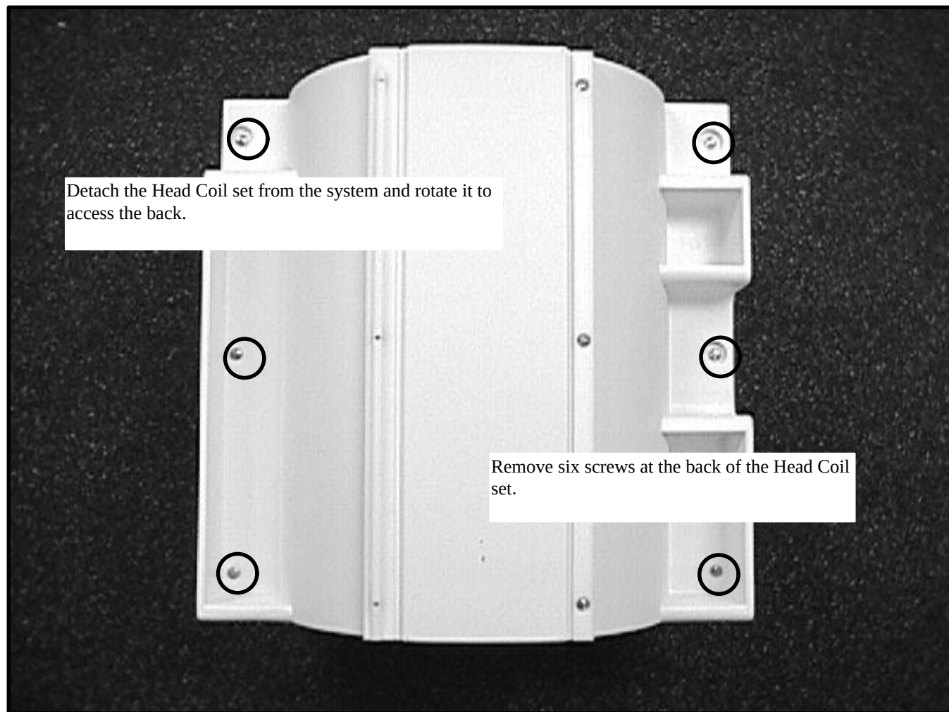
BOTTOM VIEW OF HEAD COIL ILLUSTRATION 5-1
